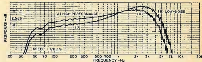
Fig. 8. Same as for Fig. 6 but at a tape speed of 1 7/8 in/s.
