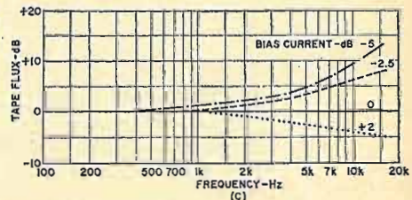
Fig. 2. (A) Frequency response with different bias currents showing the need for equalization. (B) Same as (A) but with outputs at low frequencies adjusted to same level. (C) Same as (A) but with the system equalized for a flat response when the bias has been adjusted to provide the maximum sensitivity at low signal frequencies.
