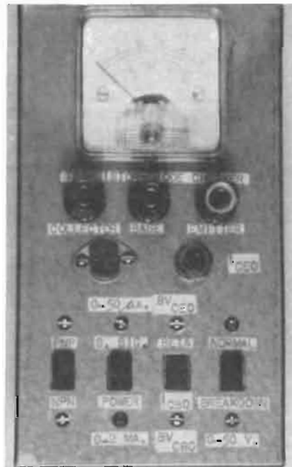
Fig. 3. (Top) The front panel of the tester. (Below) Meter scale modifications for tests.
